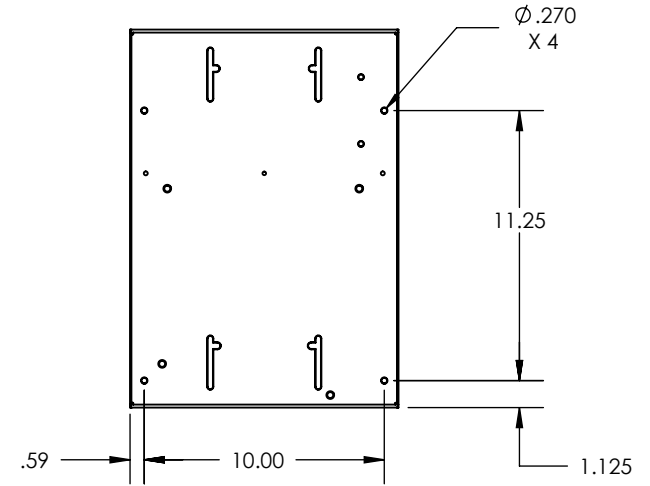
WALL MOUNTING HOLES
